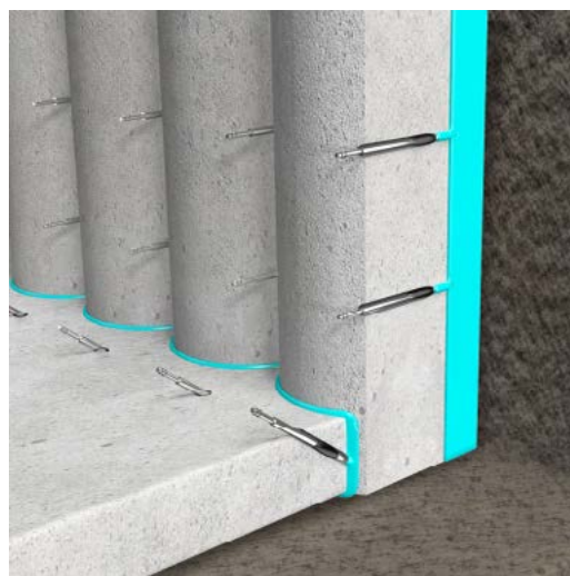
Sealing of pile head wall against pressurized water
