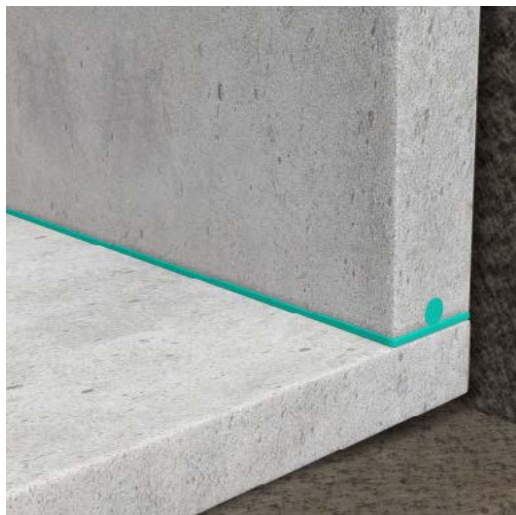
Concrete joint sealing with injection hoses and subsequent injection with injection resin
