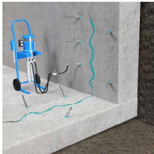
Flexible and structural crack injection into humid and dry cracks
