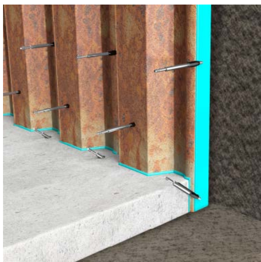
Waterproofing of sheet piling wall against pressurized water
