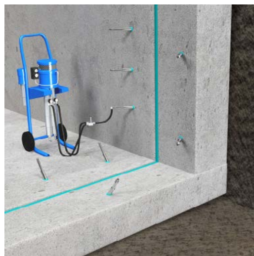
DILATATION SEALING SYSTEM The acrylic polymer injection filler is especially designed for expansion joints.
